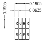
PIXEL DETAIL (SCALE 50:1)
