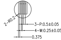
DETAIL B (SCALE 3:1)
